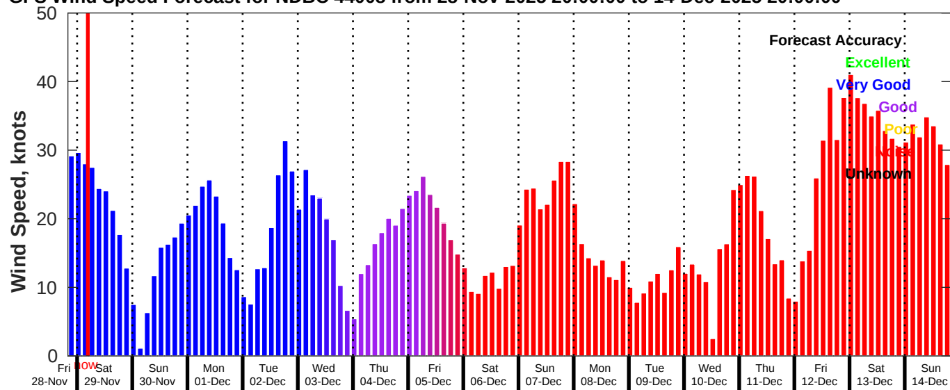
GFS Wind Speed Forecast for NDBC 44008 from 28-Nov-2025 20:00:00 to 14-Dec-2025 20:00:00
