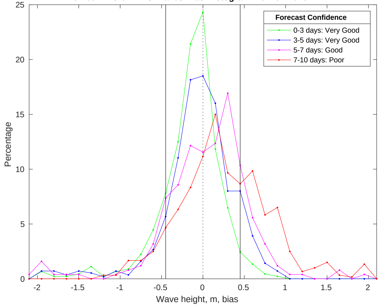
NDBC 46011 vs CMEMS Waves Bias Histogram: 29-Nov-2025
