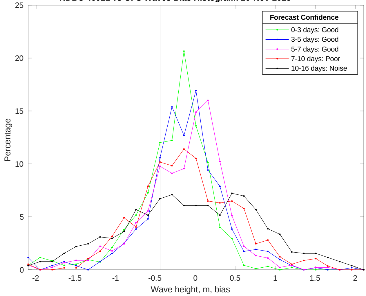
NDBC 46011 vs GFS Waves Bias Histogram: 29-Nov-2025
