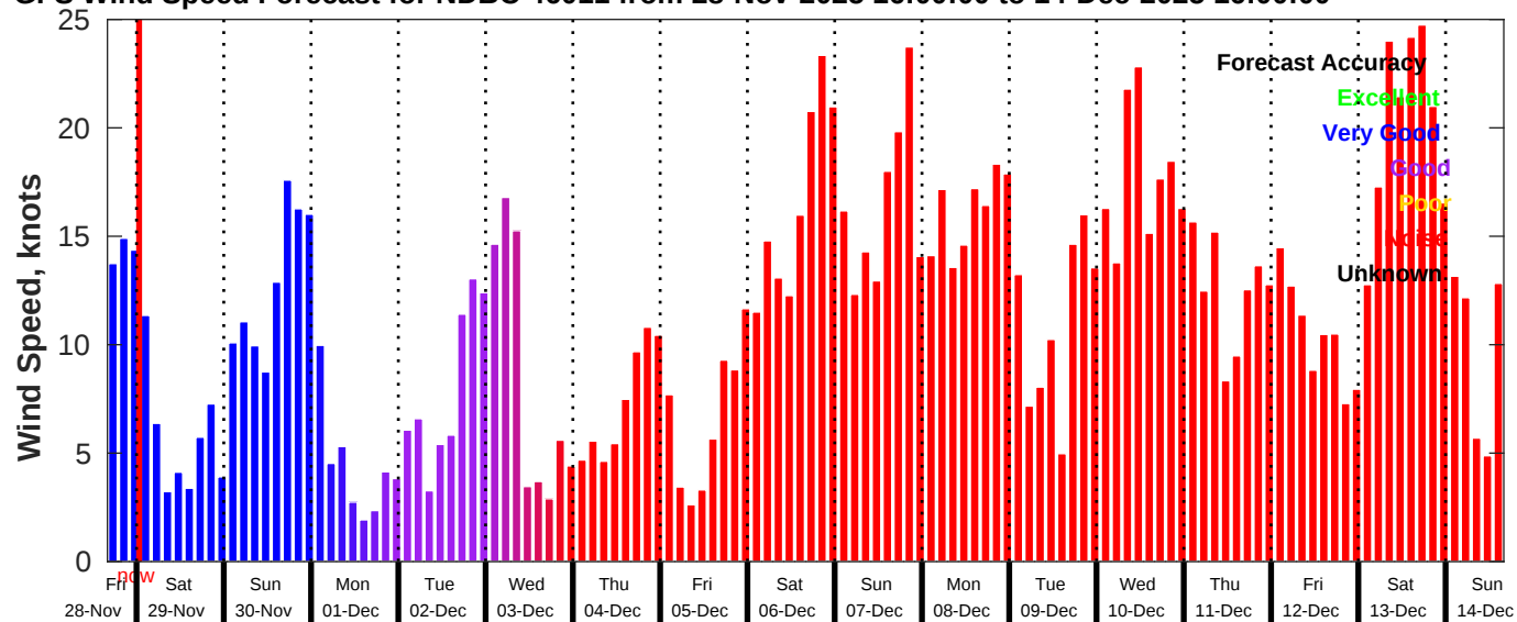
GFS Wind Speed Forecast for NDBC 46011 from 28-Nov-2025 16:00:00 to 14-Dec-2025 16:00:00
