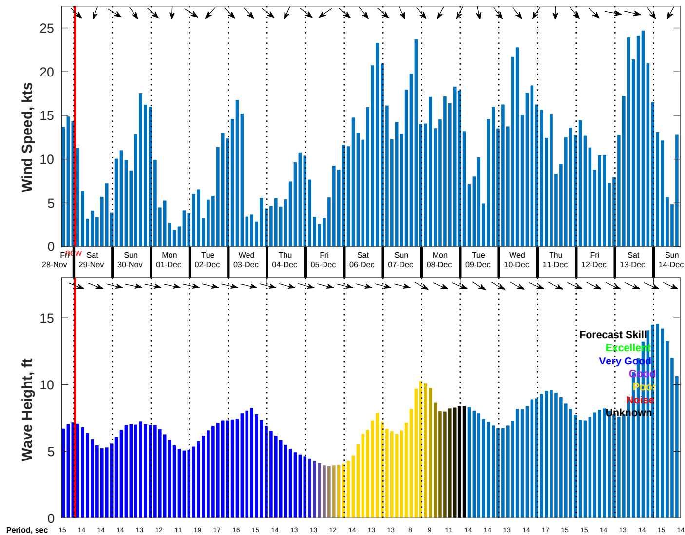
Wind & Wave Forecast for NDBC 46011 from 28-Nov-2025 16:00:00 to 14-Dec-2025 16:00:00
