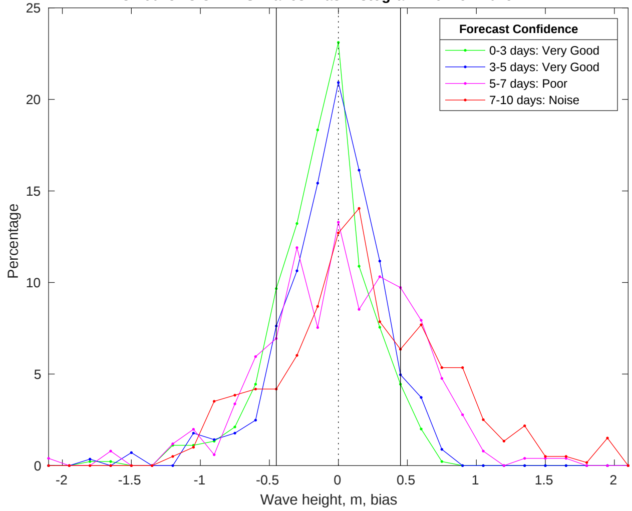
NDBC 46028 vs CMEMS Waves Bias Histogram: 29-Nov-2025
