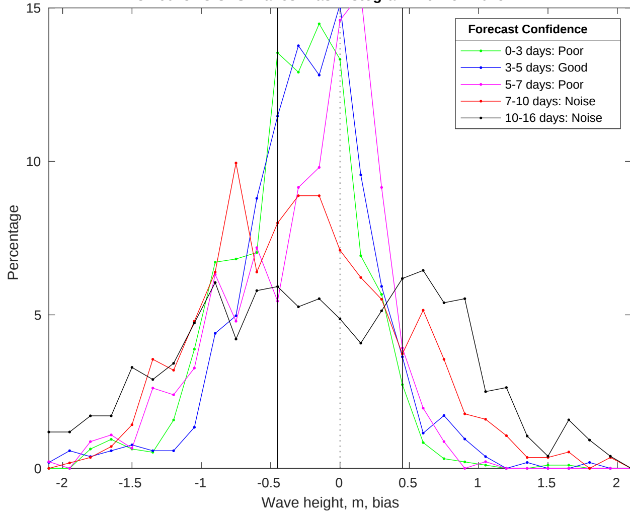
NDBC 46028 vs GFS Waves Bias Histogram: 29-Nov-2025
