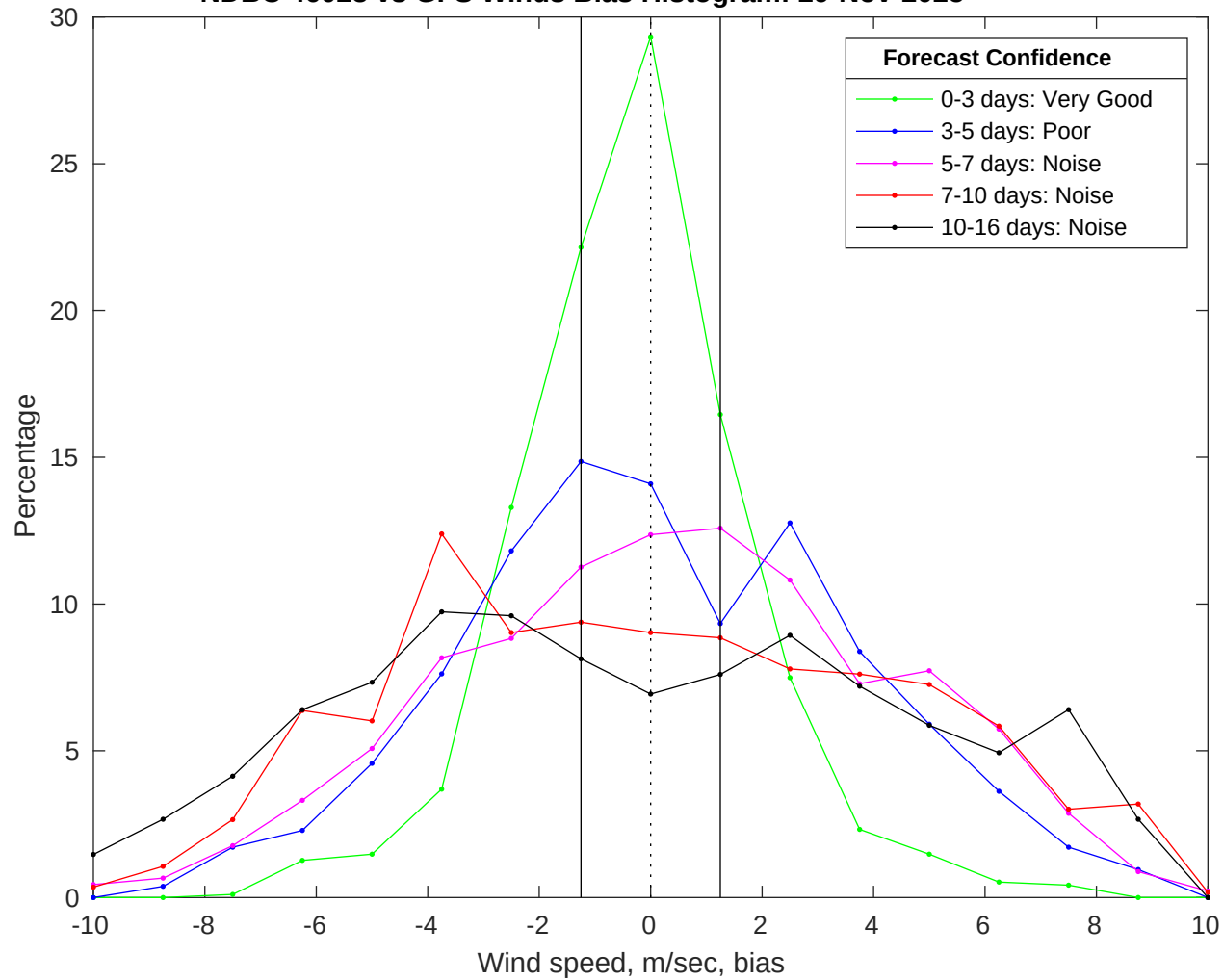
NDBC 46028 vs GFS Winds Bias Histogram: 29-Nov-2025
