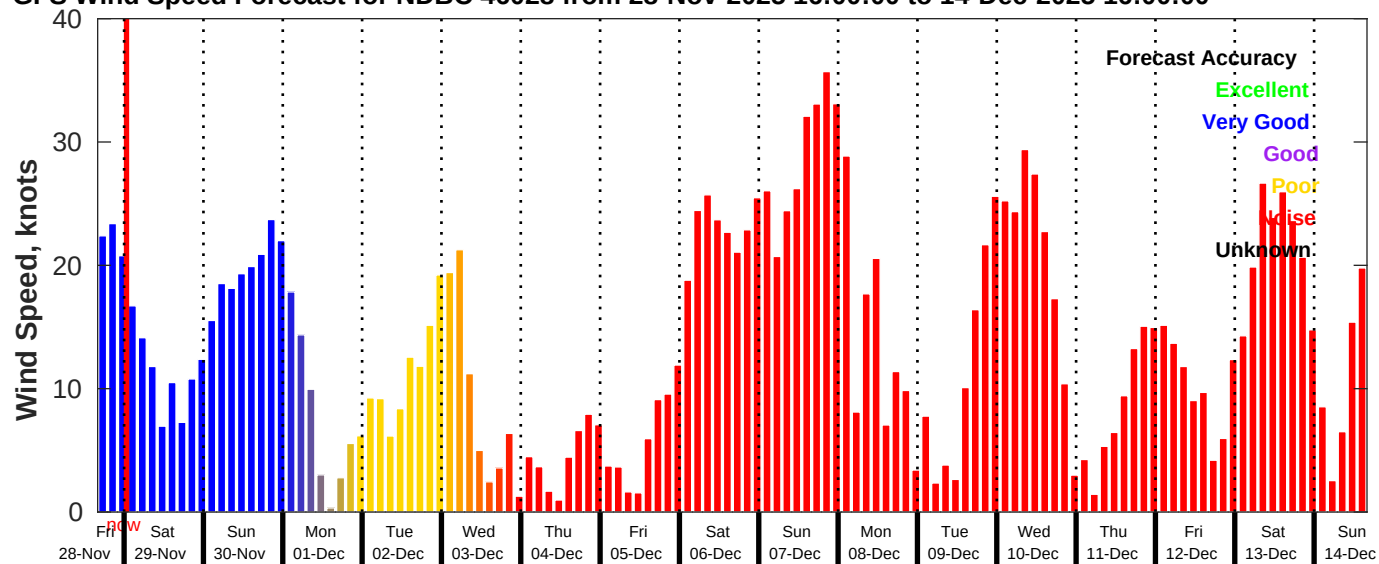
GFS Wind Speed Forecast for NDBC 46028 from 28-Nov-2025 16:00:00 to 14-Dec-2025 16:00:00
