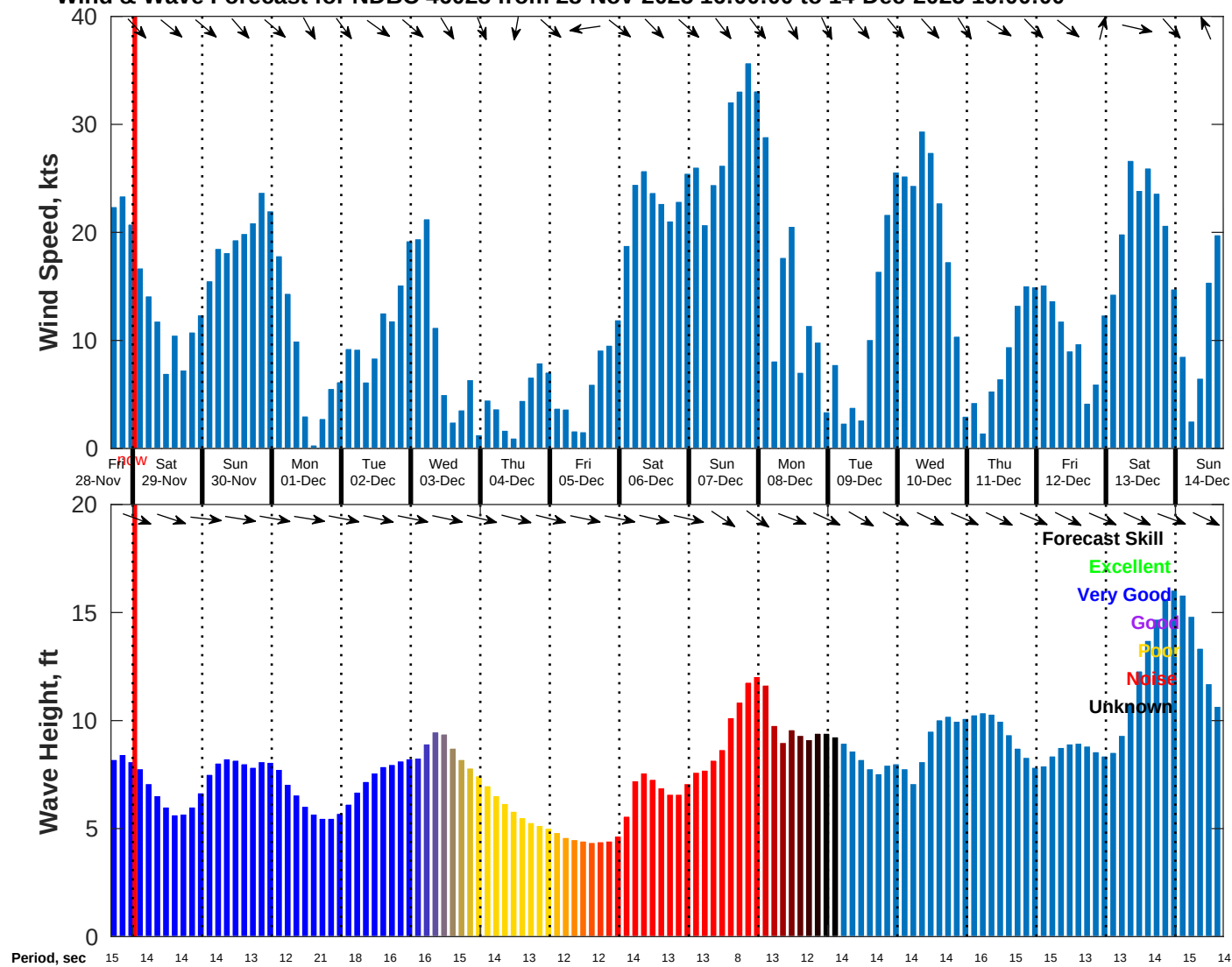
Wind & Wave Forecast for NDBC 46028 from 28-Nov-2025 16:00:00 to 14-Dec-2025 16:00:00
