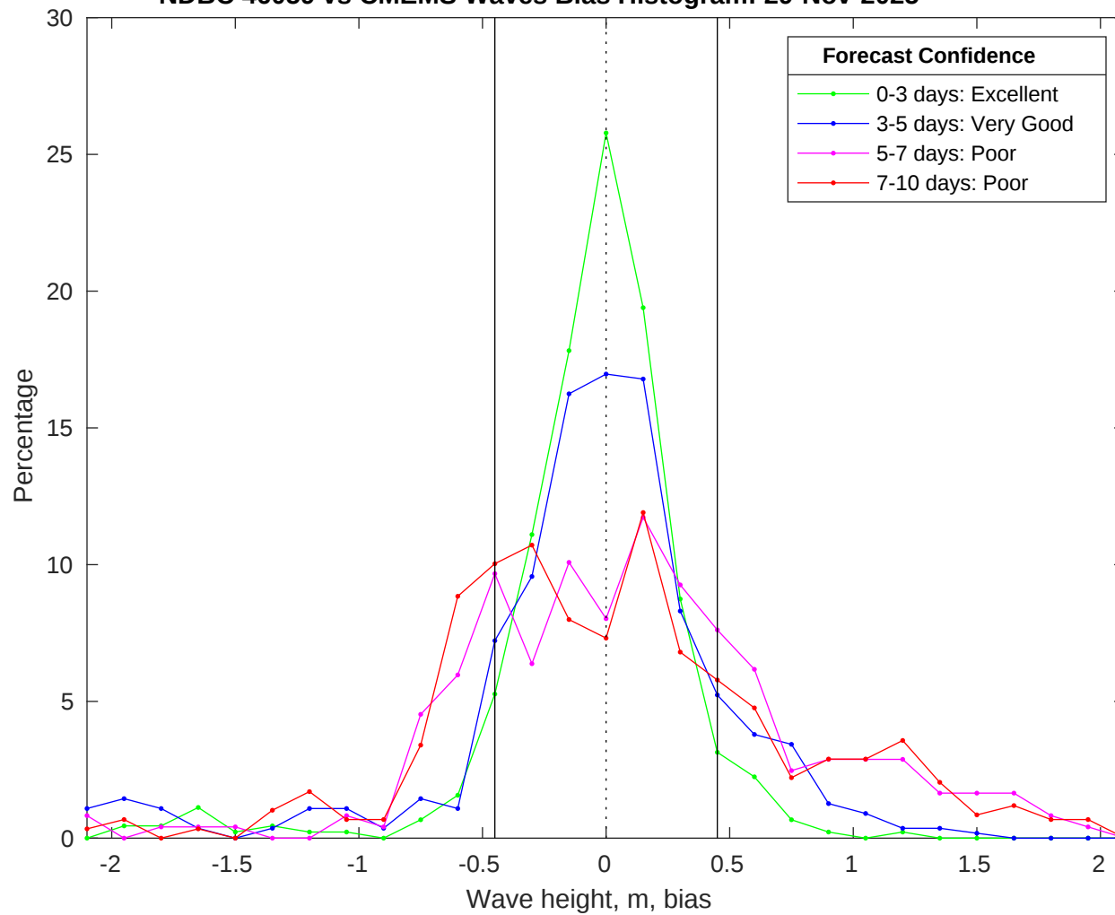
NDBC 46059 vs CMEMS Waves Bias Histogram: 29-Nov-2025
