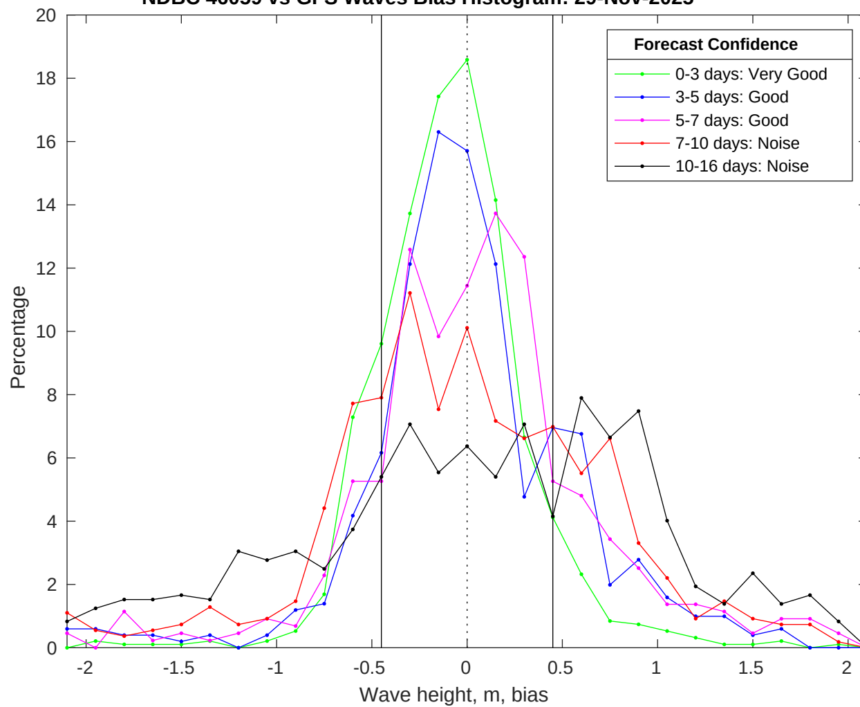
NDBC 46059 vs GFS Waves Bias Histogram: 29-Nov-2025
