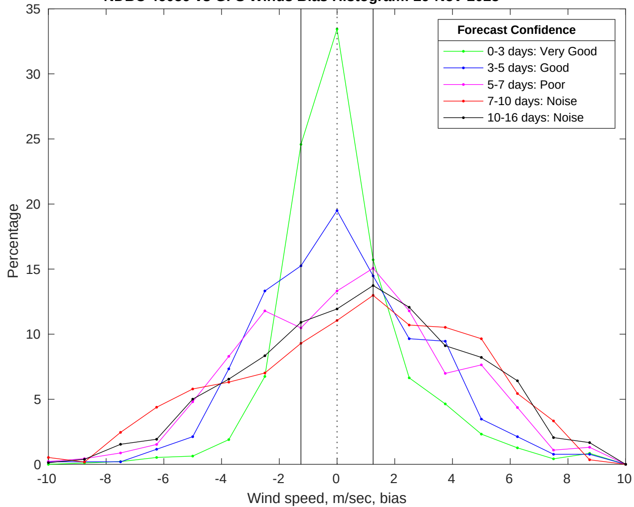
NDBC 46059 vs GFS Winds Bias Histogram: 29-Nov-2025
