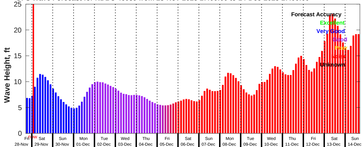
GFS Wave Forecast for NDBC 46059 from 28-Nov-2025 17:00:00 to 14-Dec-2025 17:00:00
