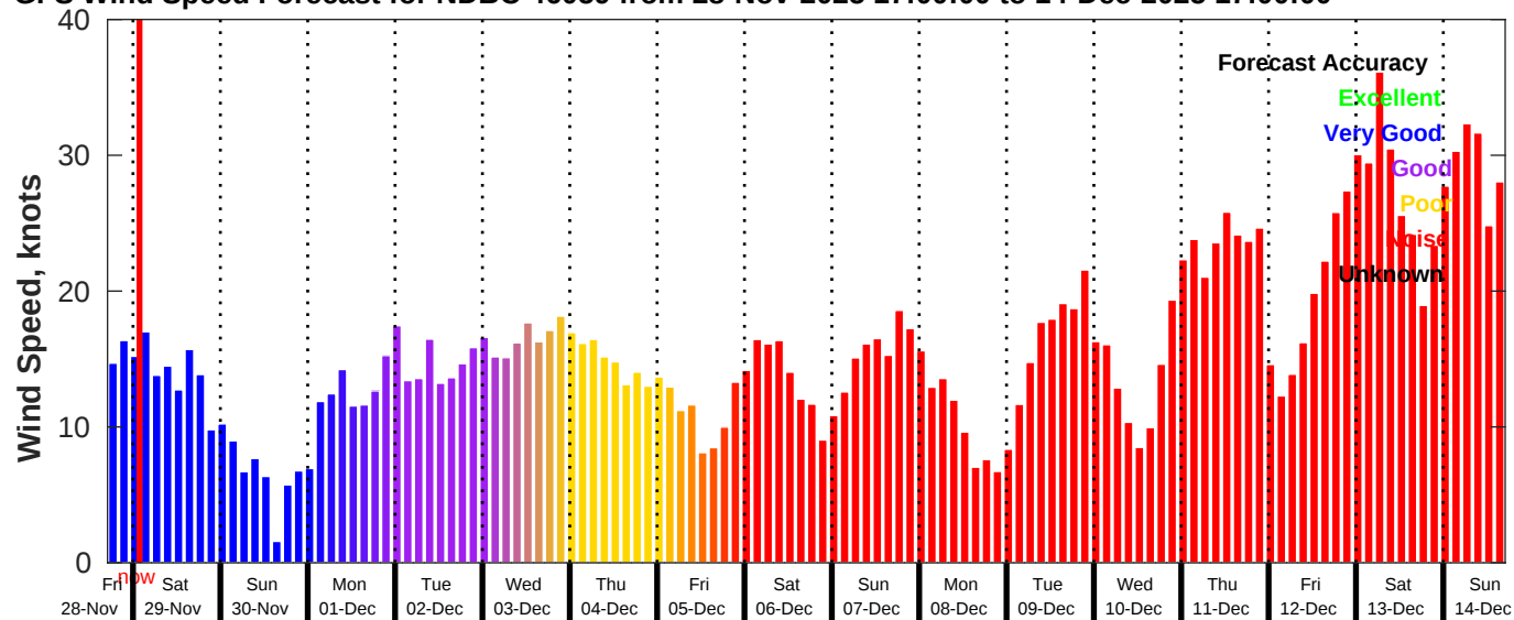
GFS Wind Speed Forecast for NDBC 46059 from 28-Nov-2025 17:00:00 to 14-Dec-2025 17:00:00
