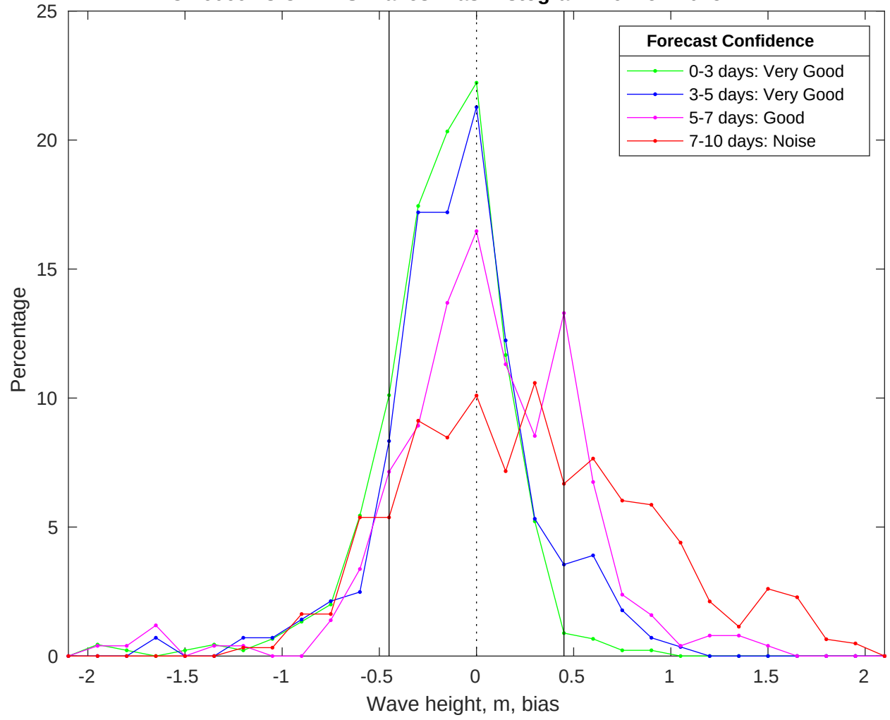
NDBC 46069 vs CMEMS Waves Bias Histogram: 29-Nov-2025
