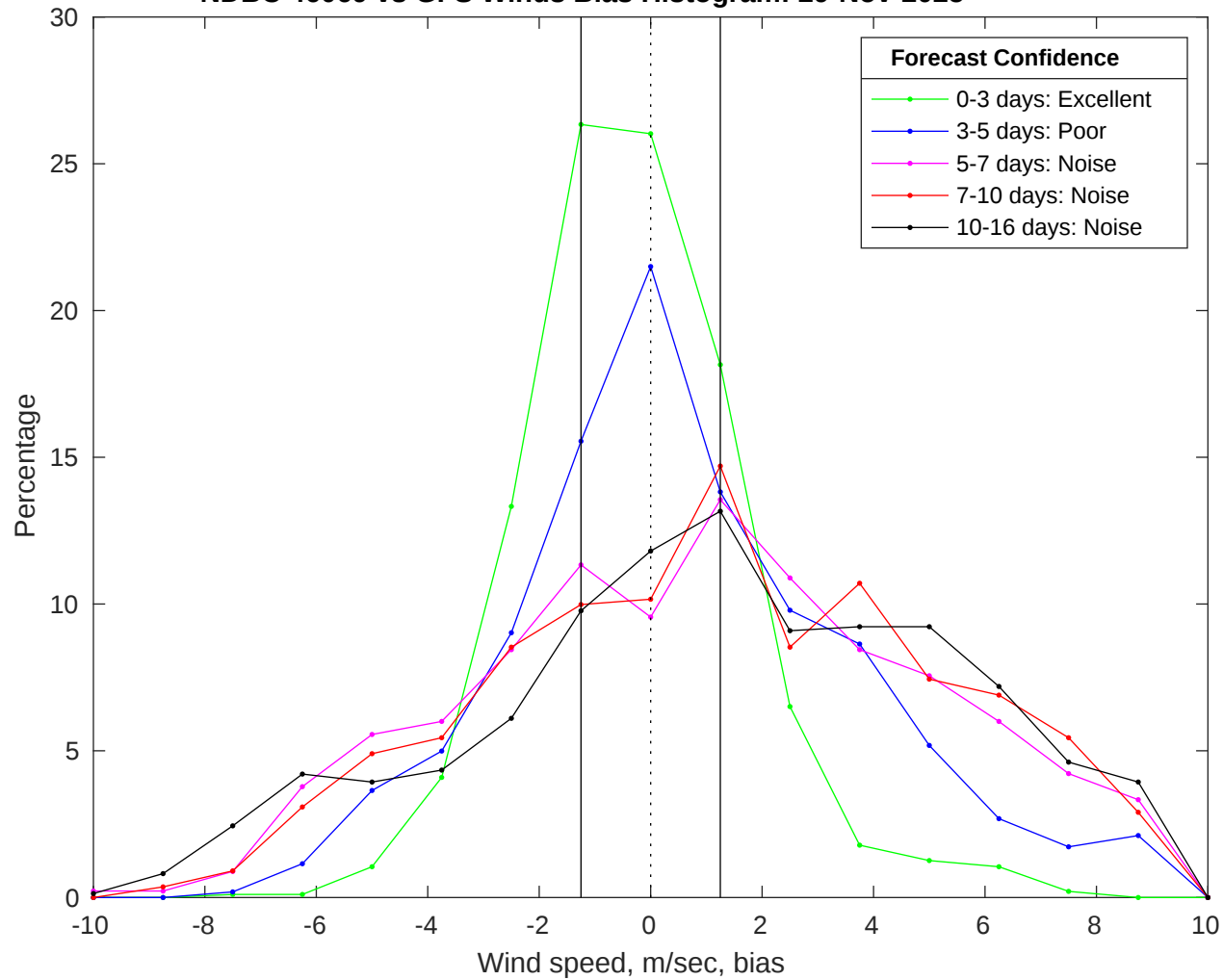
NDBC 46069 vs GFS Winds Bias Histogram: 29-Nov-2025
