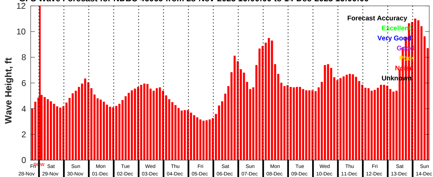
GFS Wave Forecast for NDBC 46069 from 28-Nov-2025 16:00:00 to 14-Dec-2025 16:00:00
