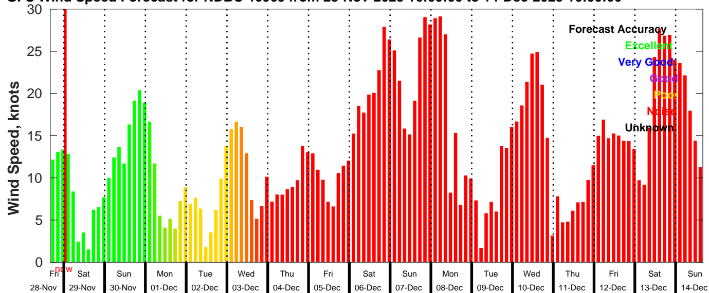
GFS Wind Speed Forecast for NDBC 46069 from 28-Nov-2025 16:00:00 to 14-Dec-2025 16:00:00
