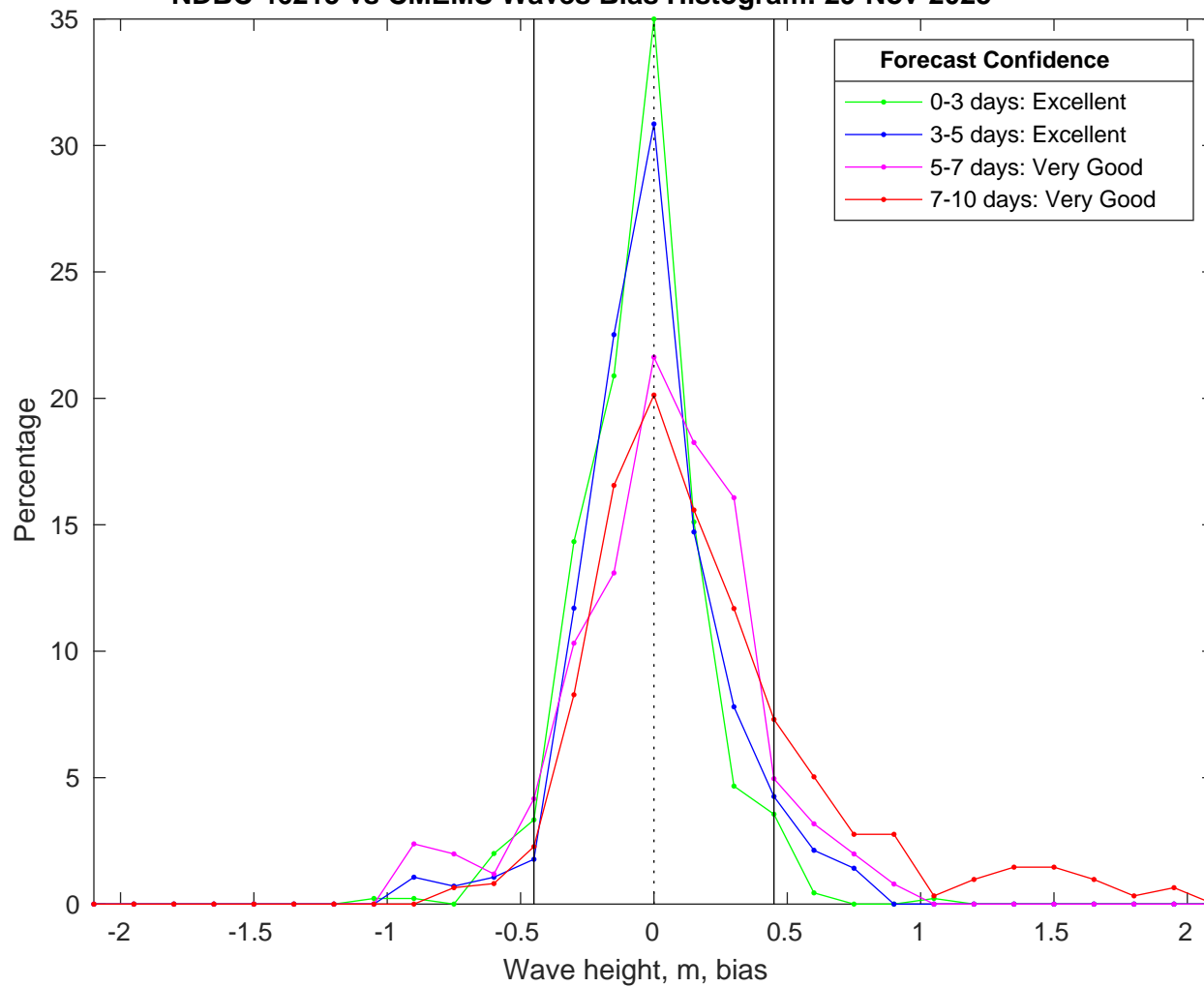
NDBC 46215 vs CMEMS Waves Bias Histogram: 29-Nov-2025
