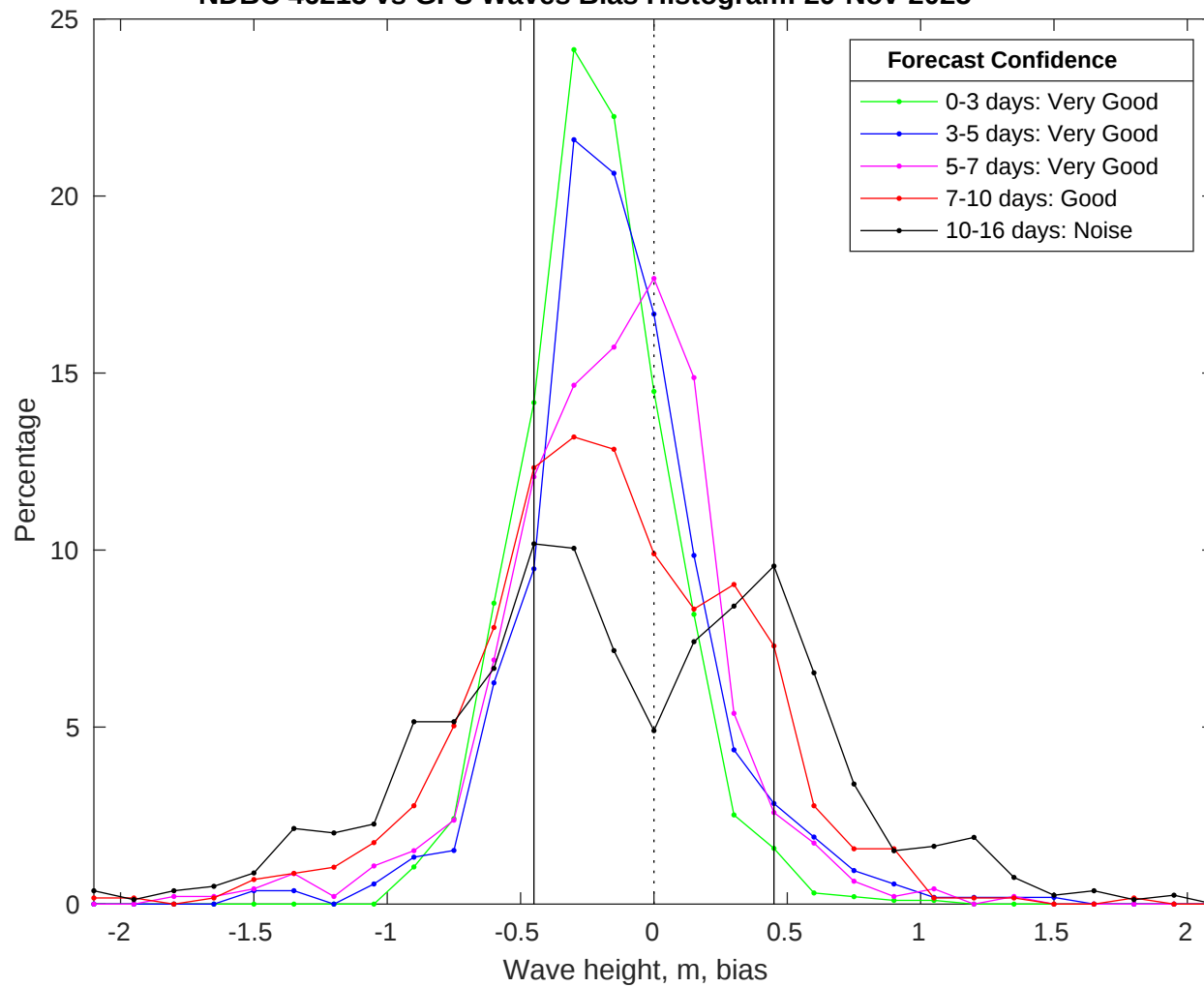
NDBC 46215 vs GFS Waves Bias Histogram: 29-Nov-2025
