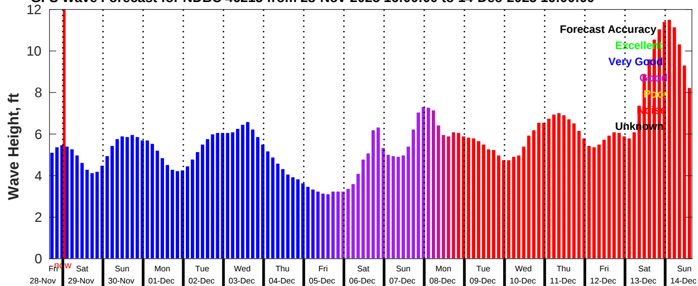
GFS Wave Forecast for NDBC 46215 from 28-Nov-2025 16:00:00 to 14-Dec-2025 16:00:00
