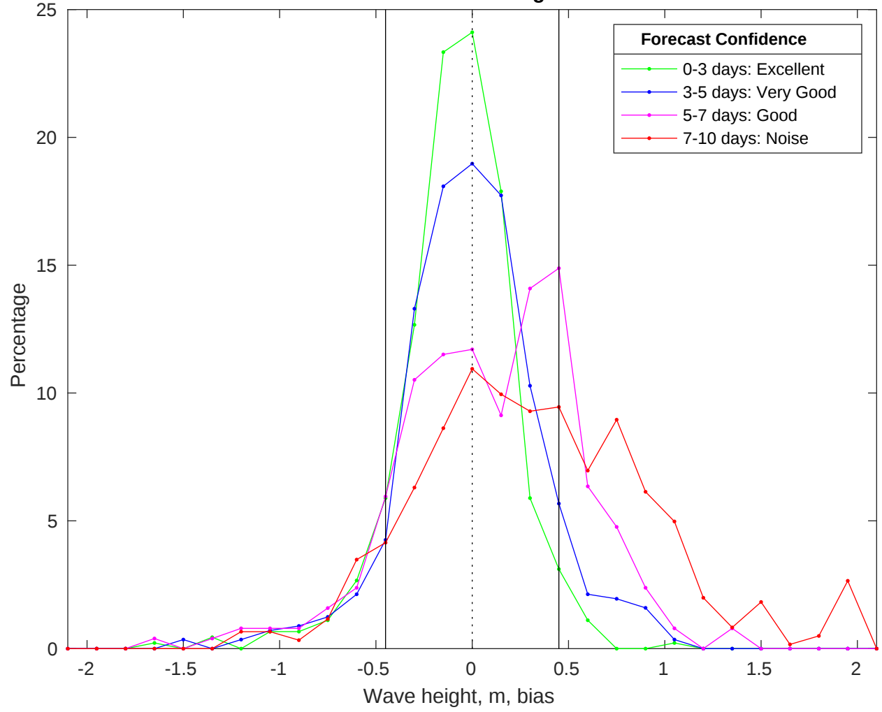
NDBC 46259 vs CMEMS Waves Bias Histogram: 29-Nov-2025
