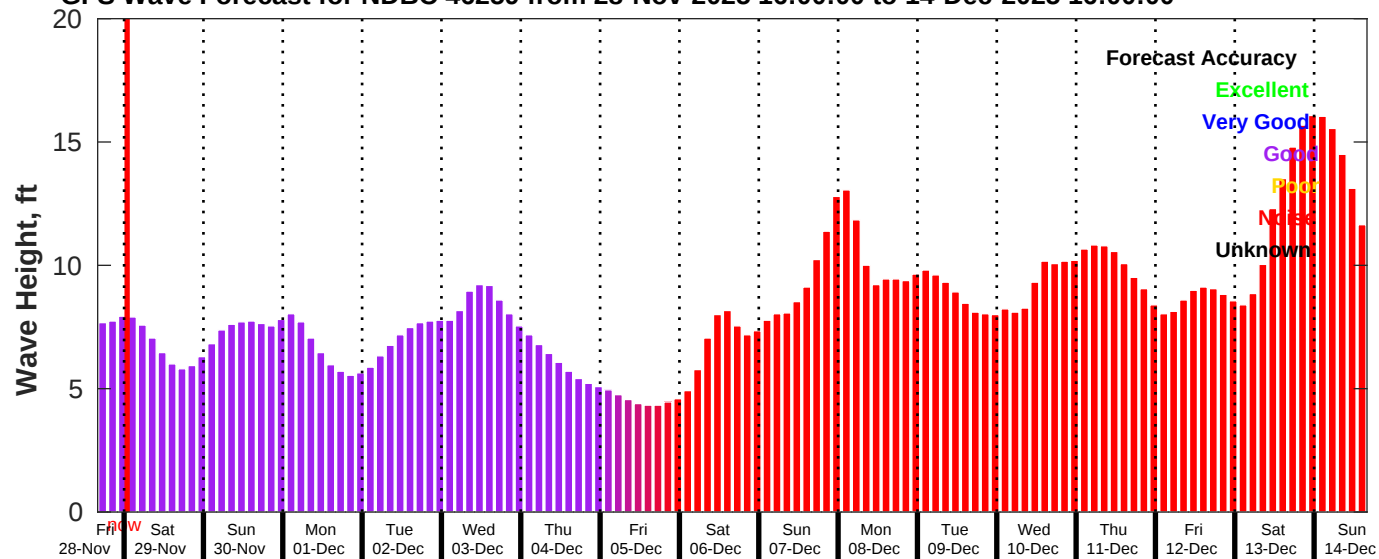
GFS Wave Forecast for NDBC 46259 from 28-Nov-2025 16:00:00 to 14-Dec-2025 16:00:00
