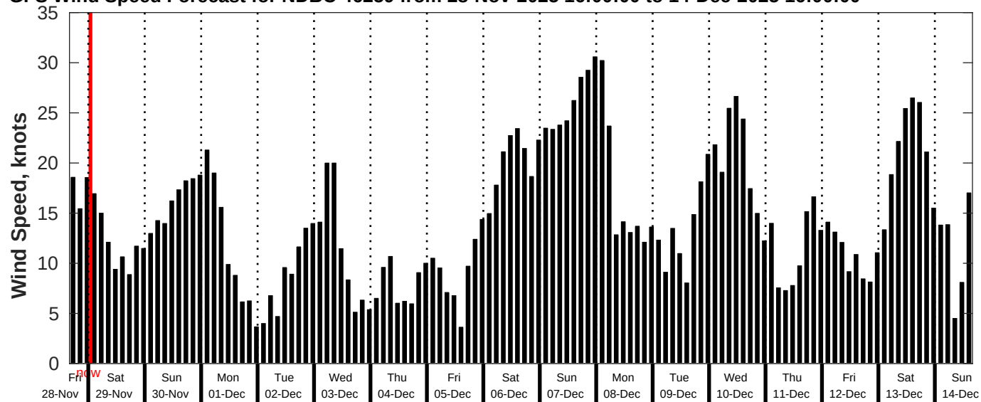
GFS Wind Speed Forecast for NDBC 46259 from 28-Nov-2025 16:00:00 to 14-Dec-2025 16:00:00
