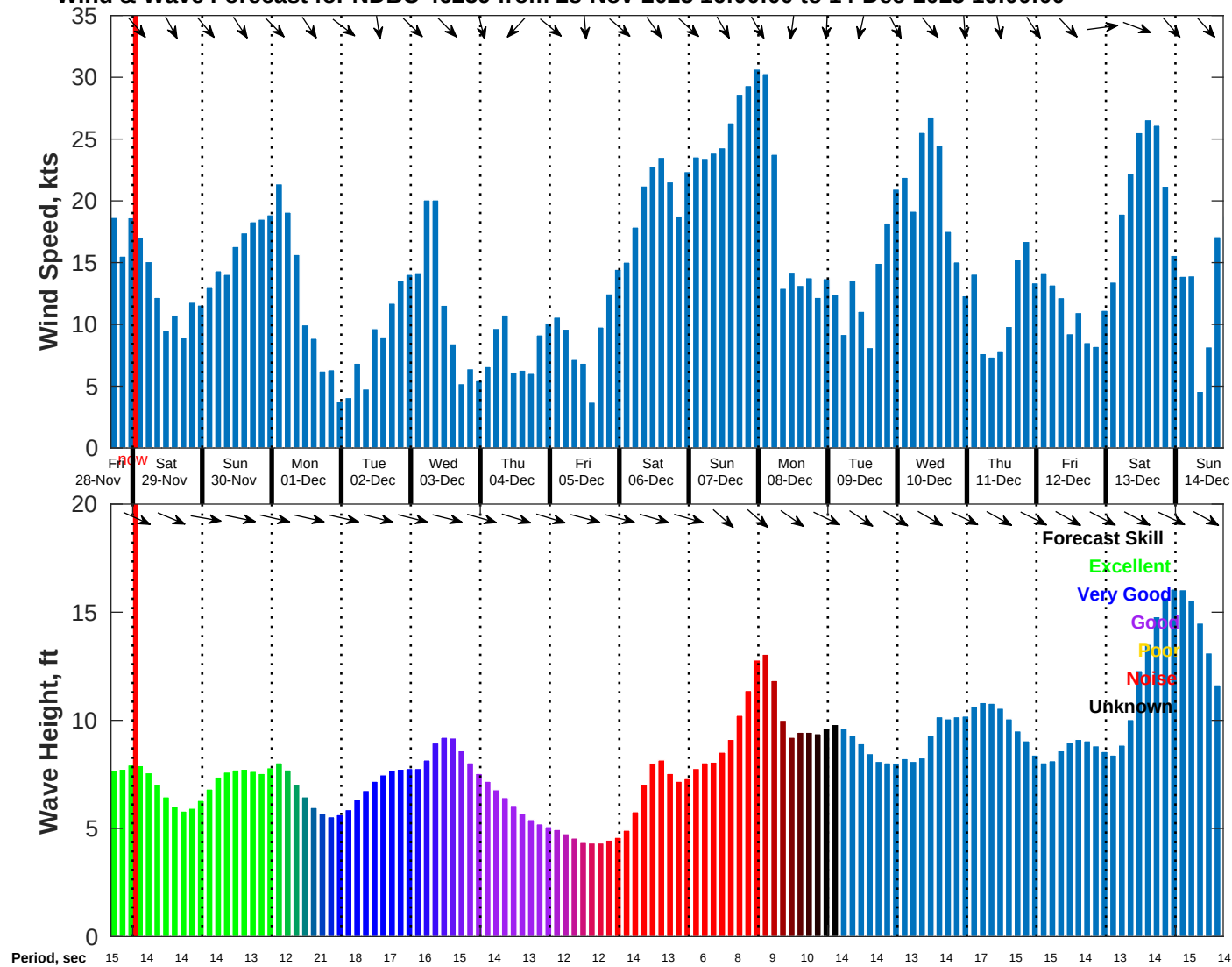
Wind & Wave Forecast for NDBC 46259 from 28-Nov-2025 16:00:00 to 14-Dec-2025 16:00:00
