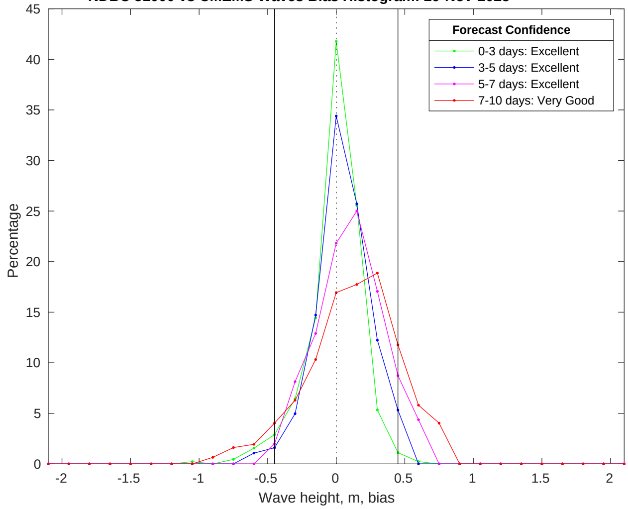
NDBC 51000 vs CMEMS Waves Bias Histogram: 29-Nov-2025
