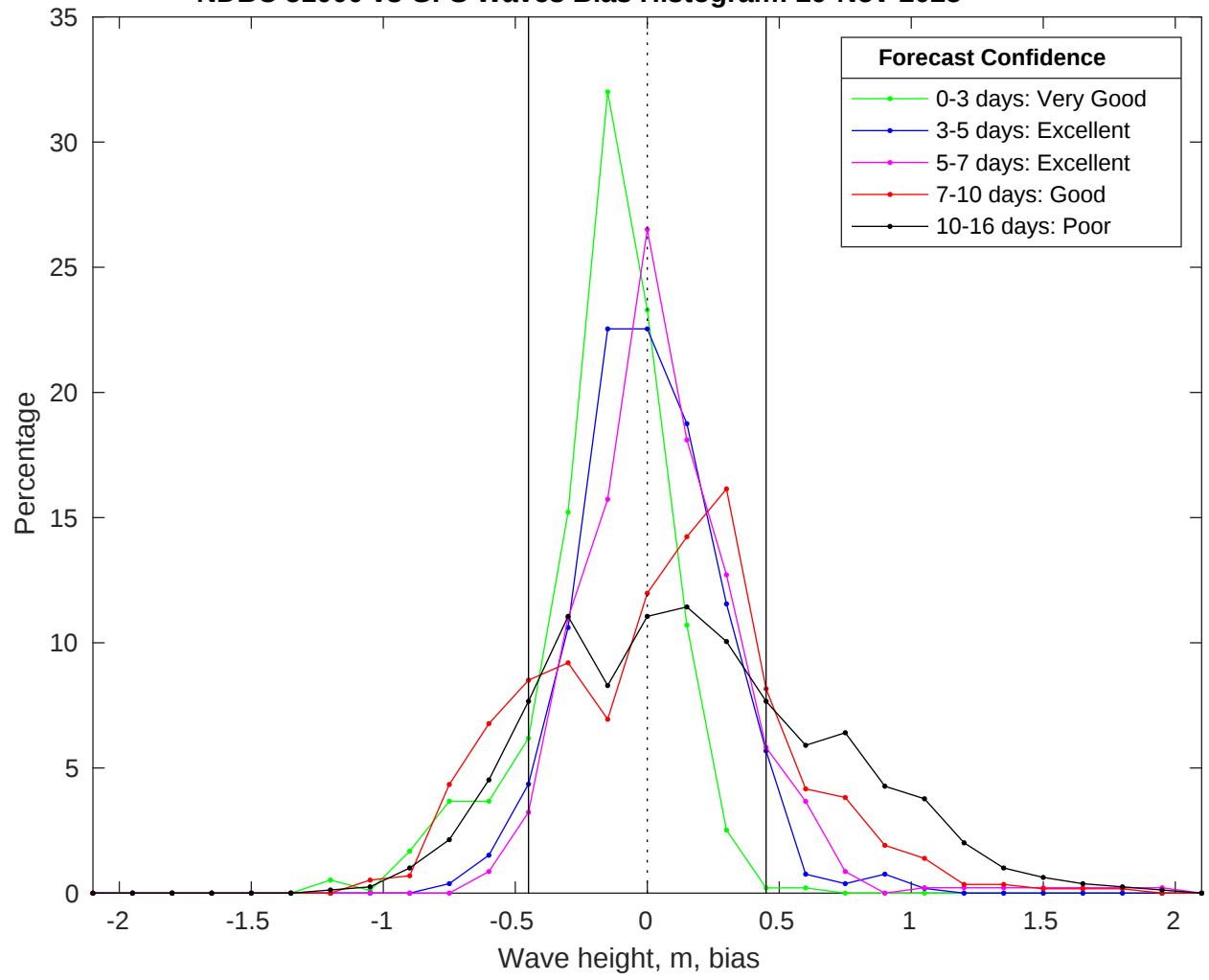
NDBC 51000 vs GFS Waves Bias Histogram: 29-Nov-2025
