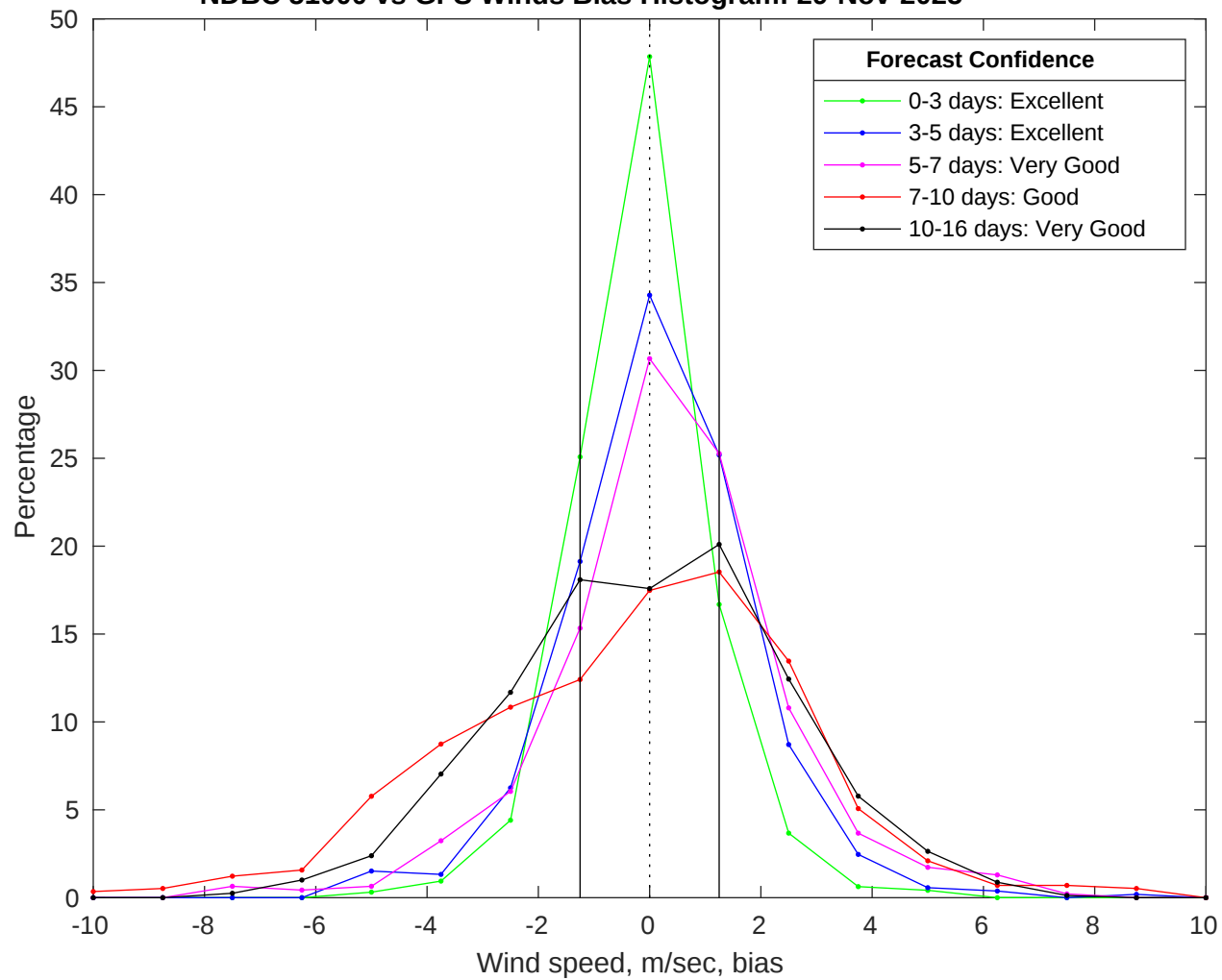
NDBC 51000 vs GFS Winds Bias Histogram: 29-Nov-2025
