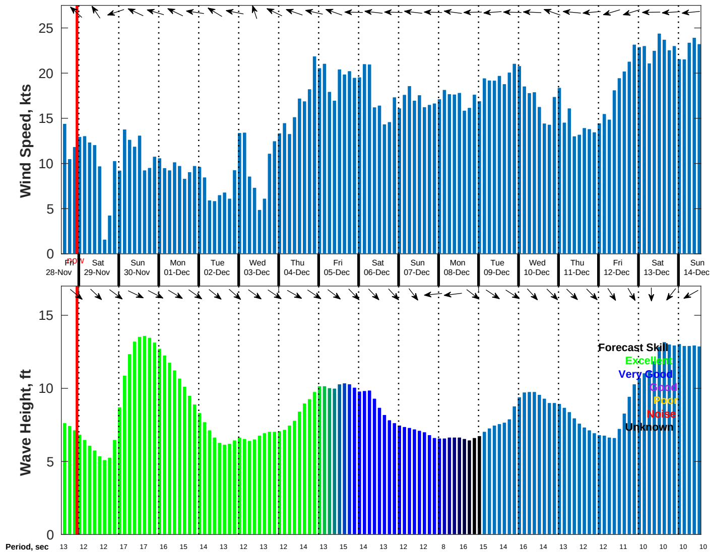
Wind & Wave Forecast for NDBC 51000 from 28-Nov-2025 14:00:00 to 14-Dec-2025 14:00:00
