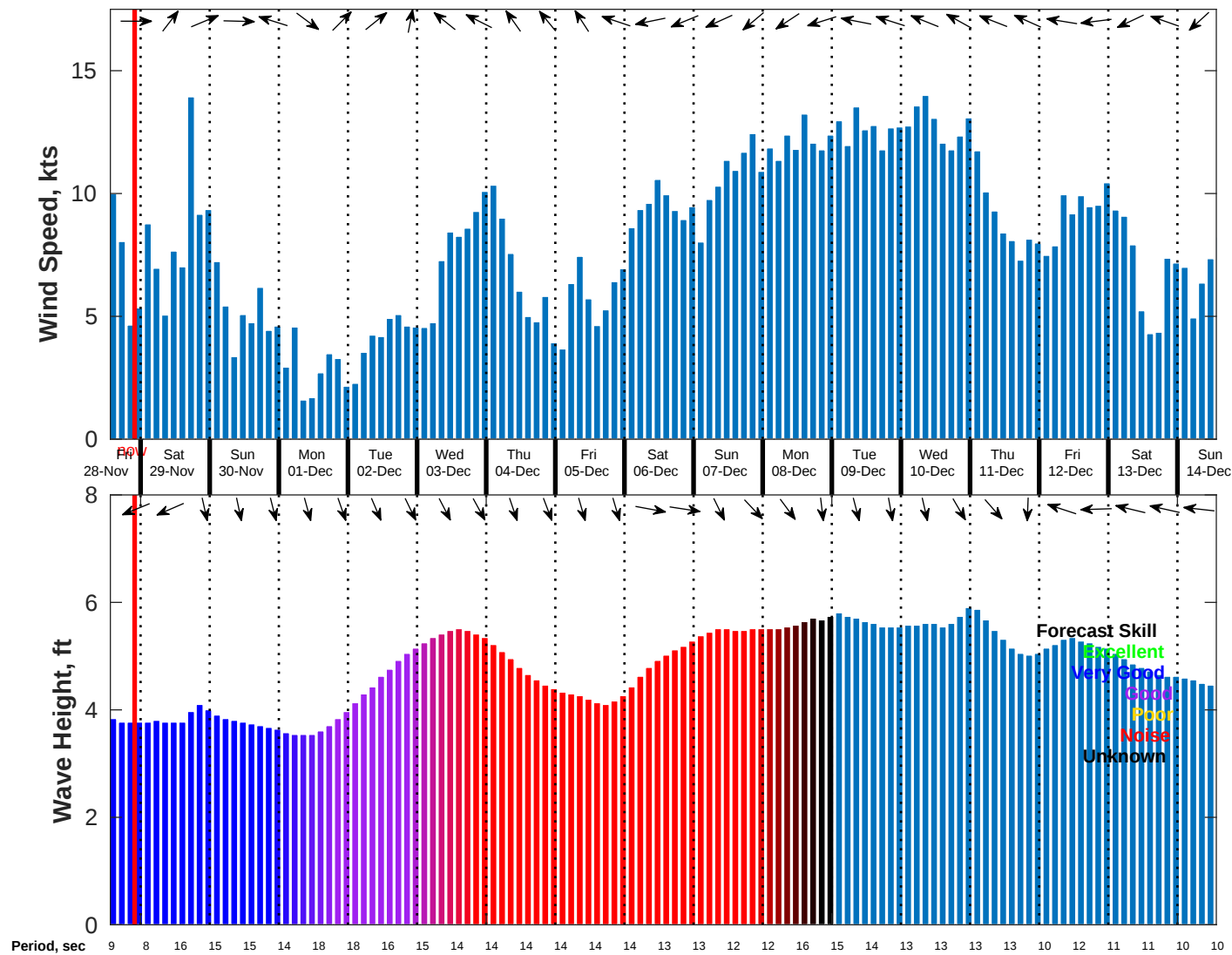
Wind & Wave Forecast for NDBC 51209 from 28-Nov-2025 13:00:00 to 14-Dec-2025 13:00:00
