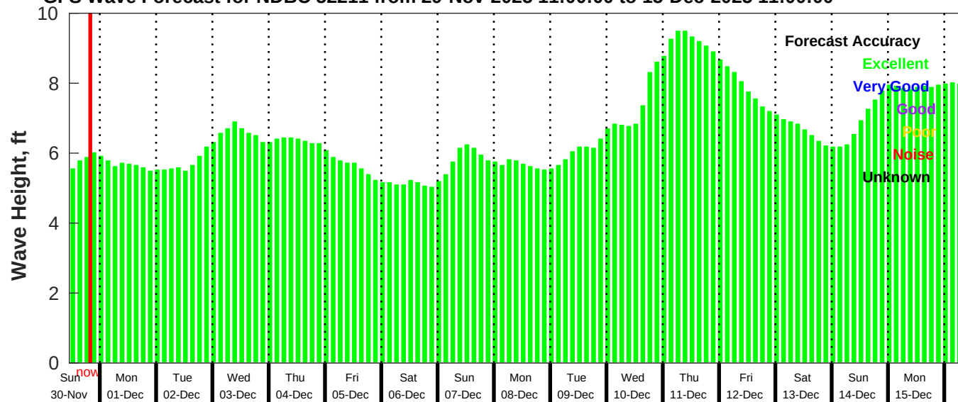
GFS Wave Forecast for NDBC 52211 from 29-Nov-2025 11:00:00 to 15-Dec-2025 11:00:00
