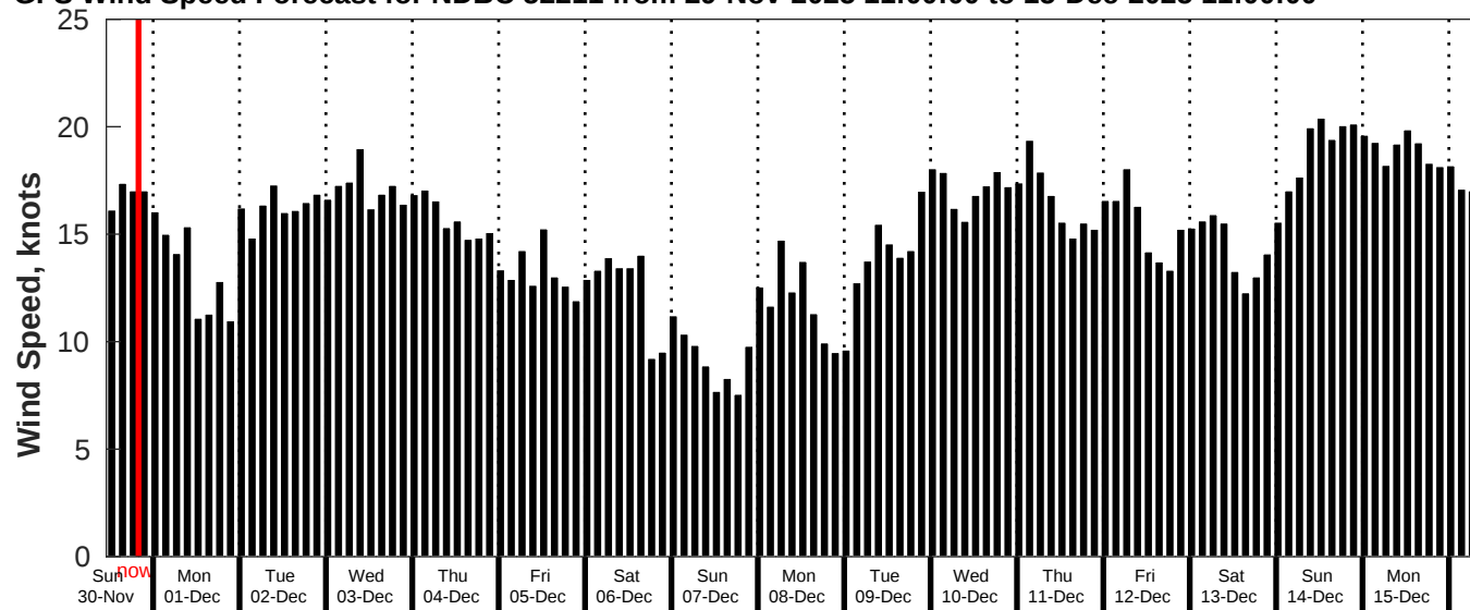
GFS Wind Speed Forecast for NDBC 52211 from 29-Nov-2025 11:00:00 to 15-Dec-2025 11:00:00
