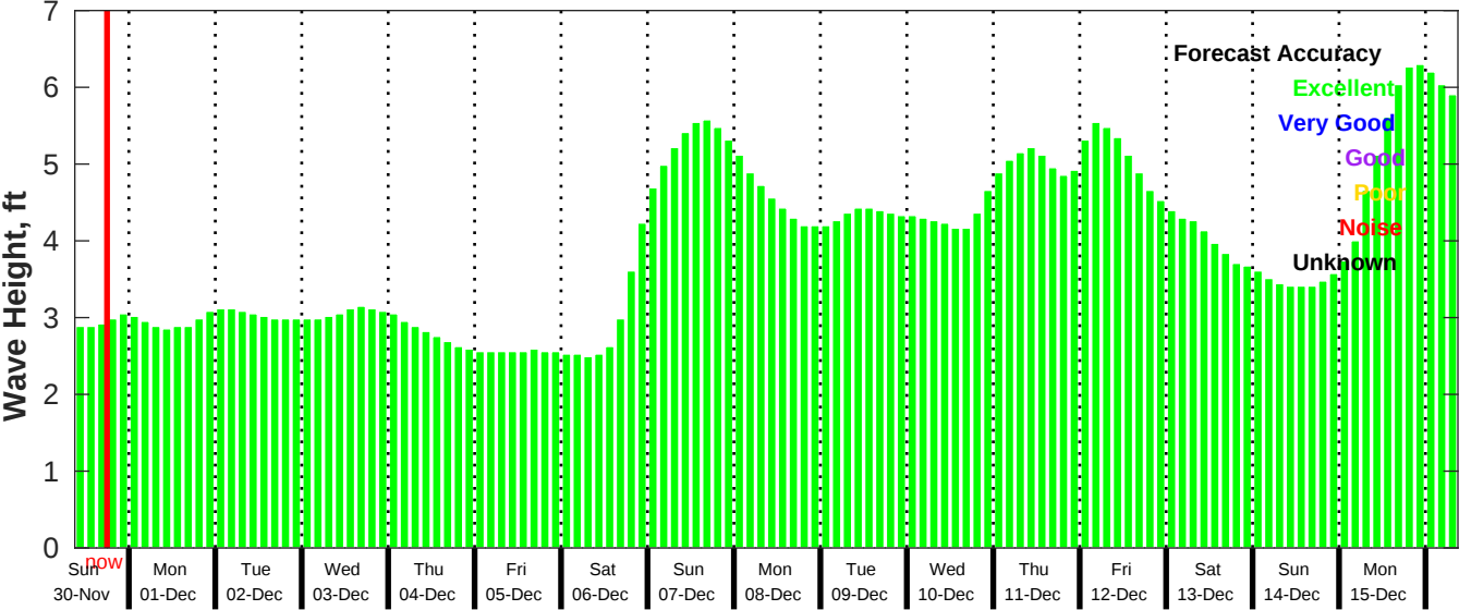
GFS Wave Forecast for NDBC 52212 from 29-Nov-2025 09:00:00 to 15-Dec-2025 09:00:00
