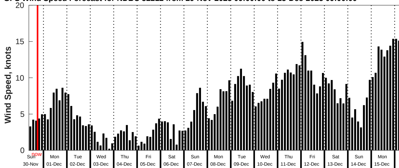
GFS Wind Speed Forecast for NDBC 52212 from 29-Nov-2025 09:00:00 to 15-Dec-2025 09:00:00
