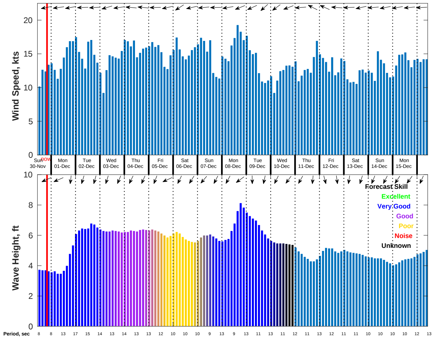
Wind & Wave Forecast for NDBC 52213 from 29-Nov-2025 11:00:00 to 15-Dec-2025 11:00:00
