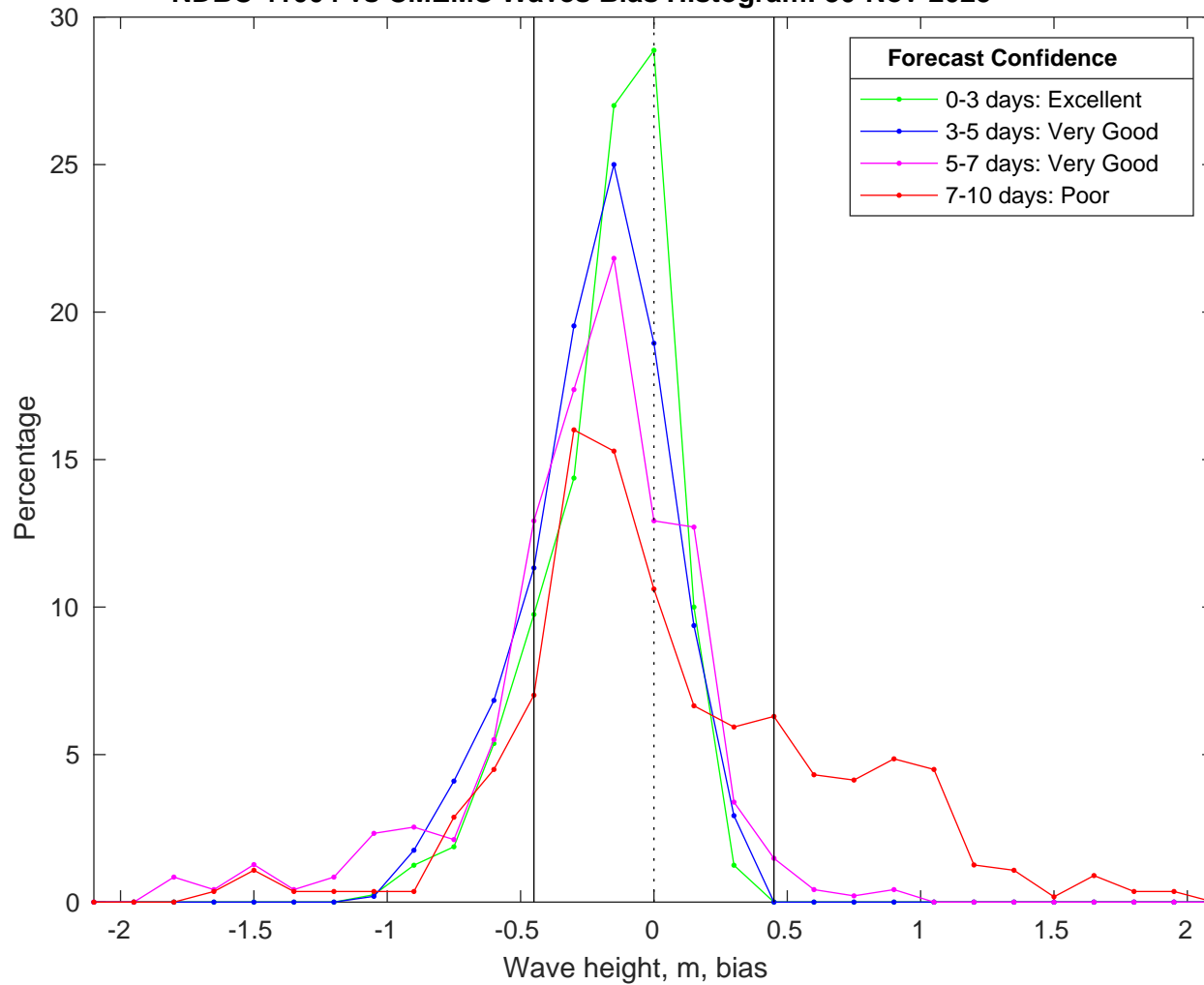
NDBC 41004 vs CMEMS Waves Bias Histogram: 30-Nov-2025
