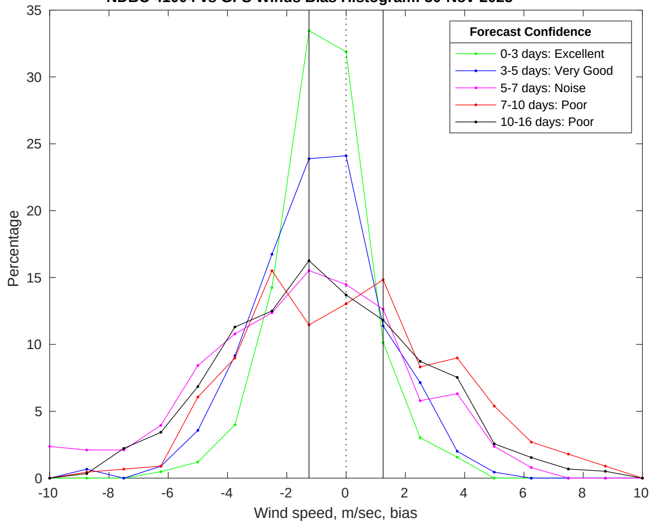
NDBC 41004 vs GFS Winds Bias Histogram: 30-Nov-2025
