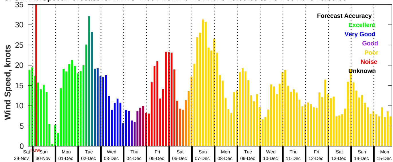
GFS Wind Speed Forecast for NDBC 41004 from 29-Nov-2025 19:00:00 to 15-Dec-2025 19:00:00
