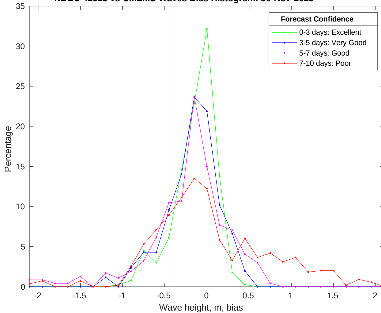
NDBC 41013 vs CMEMS Waves Bias Histogram: 30-Nov-2025
