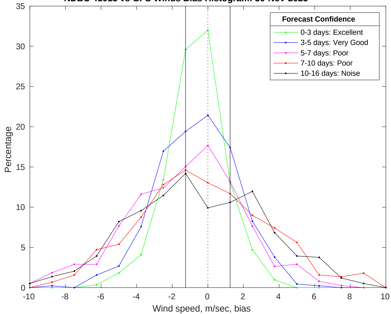
NDBC 41013 vs GFS Winds Bias Histogram: 30-Nov-2025
