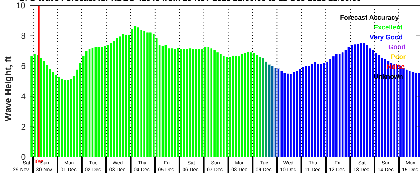
GFS Wave Forecast for NDBC 41040 from 29-Nov-2025 21:00:00 to 15-Dec-2025 21:00:00
