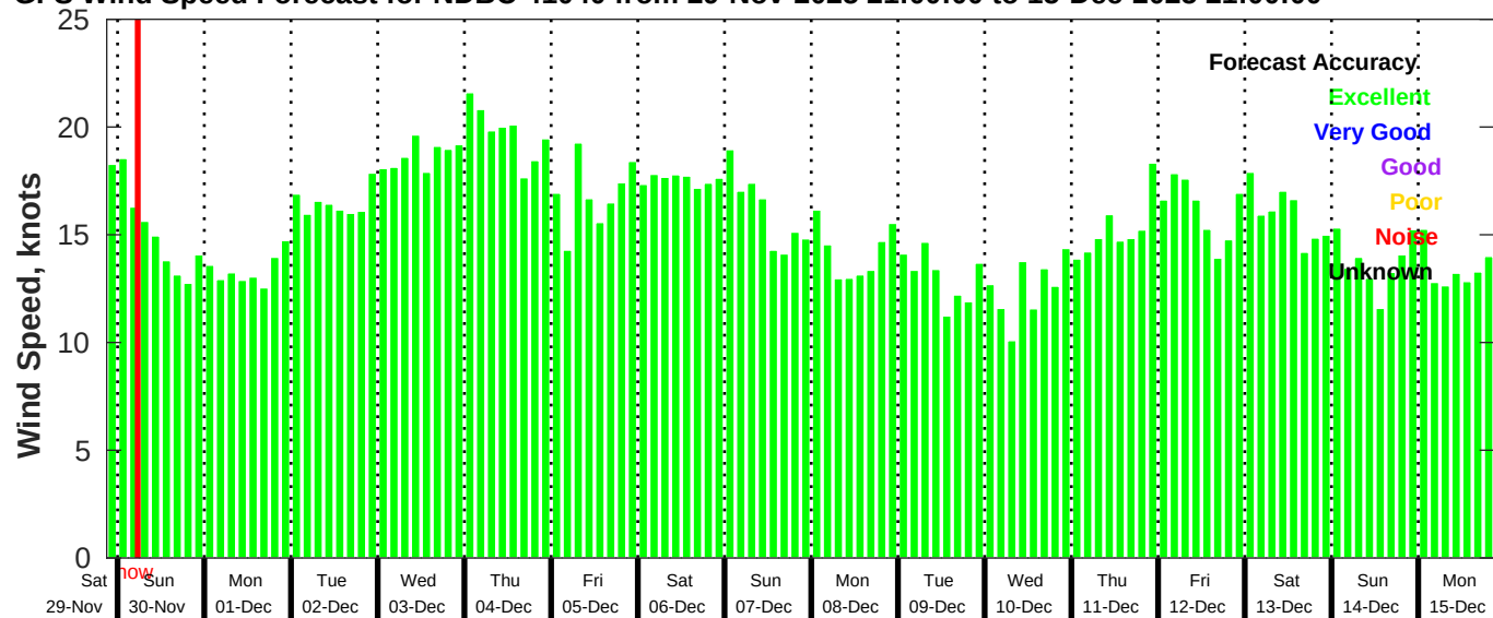
GFS Wind Speed Forecast for NDBC 41040 from 29-Nov-2025 21:00:00 to 15-Dec-2025 21:00:00
