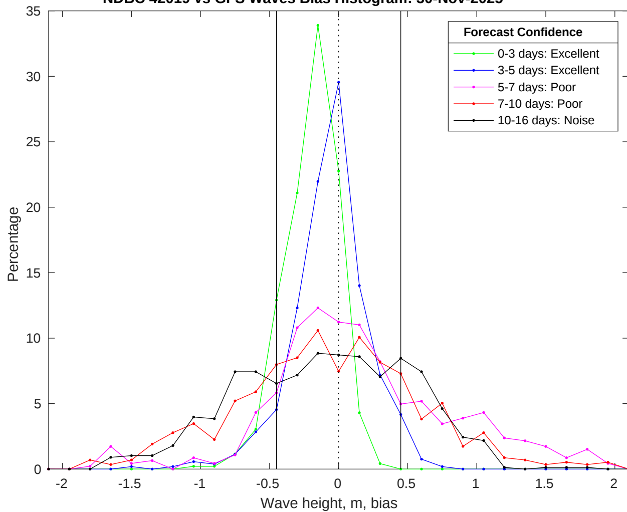
NDBC 42019 vs GFS Waves Bias Histogram: 30-Nov-2025
