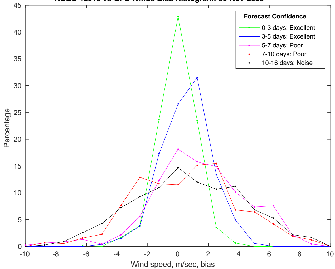
NDBC 42019 vs GFS Winds Bias Histogram: 30-Nov-2025
