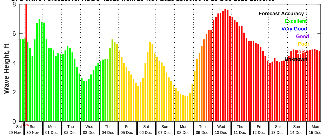
GFS Wave Forecast for NDBC 42019 from 29-Nov-2025 18:00:00 to 15-Dec-2025 18:00:00
