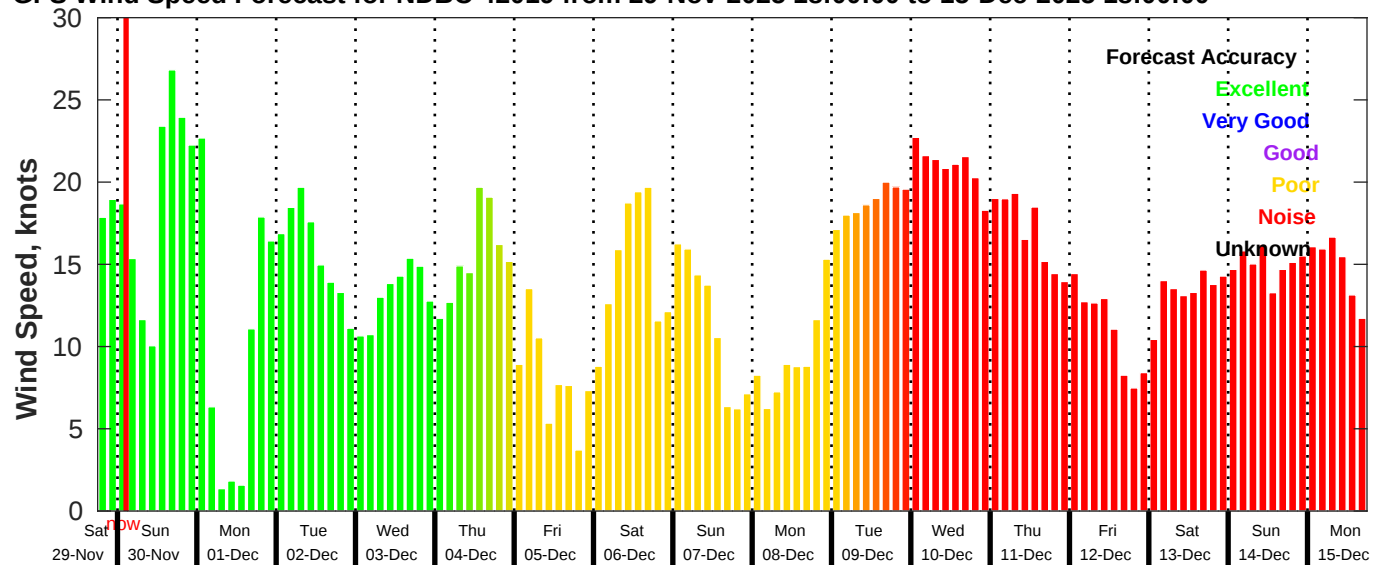
GFS Wind Speed Forecast for NDBC 42019 from 29-Nov-2025 18:00:00 to 15-Dec-2025 18:00:00
