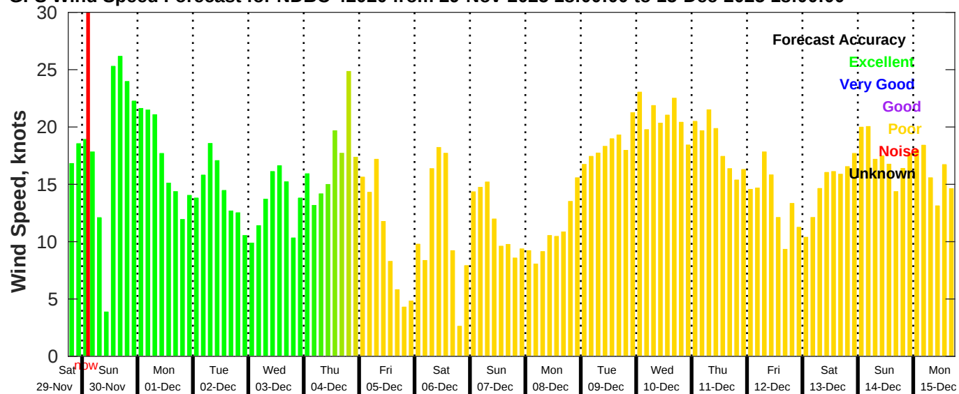
GFS Wind Speed Forecast for NDBC 42020 from 29-Nov-2025 18:00:00 to 15-Dec-2025 18:00:00
