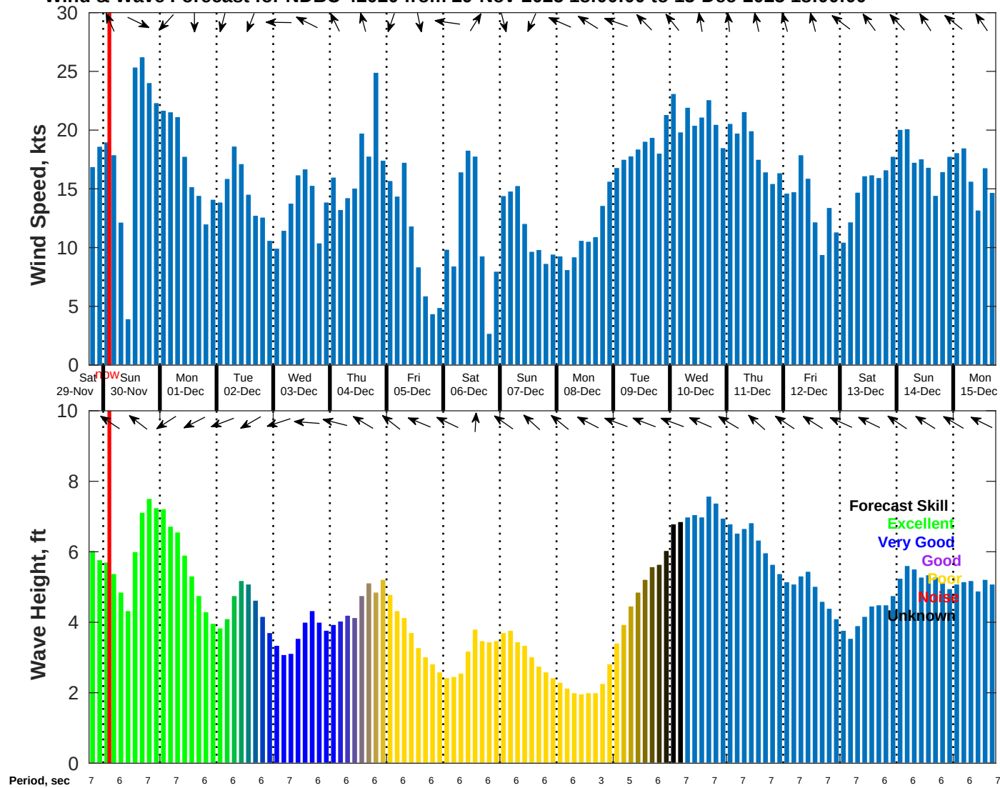
Wind & Wave Forecast for NDBC 42020 from 29-Nov-2025 18:00:00 to 15-Dec-2025 18:00:00
