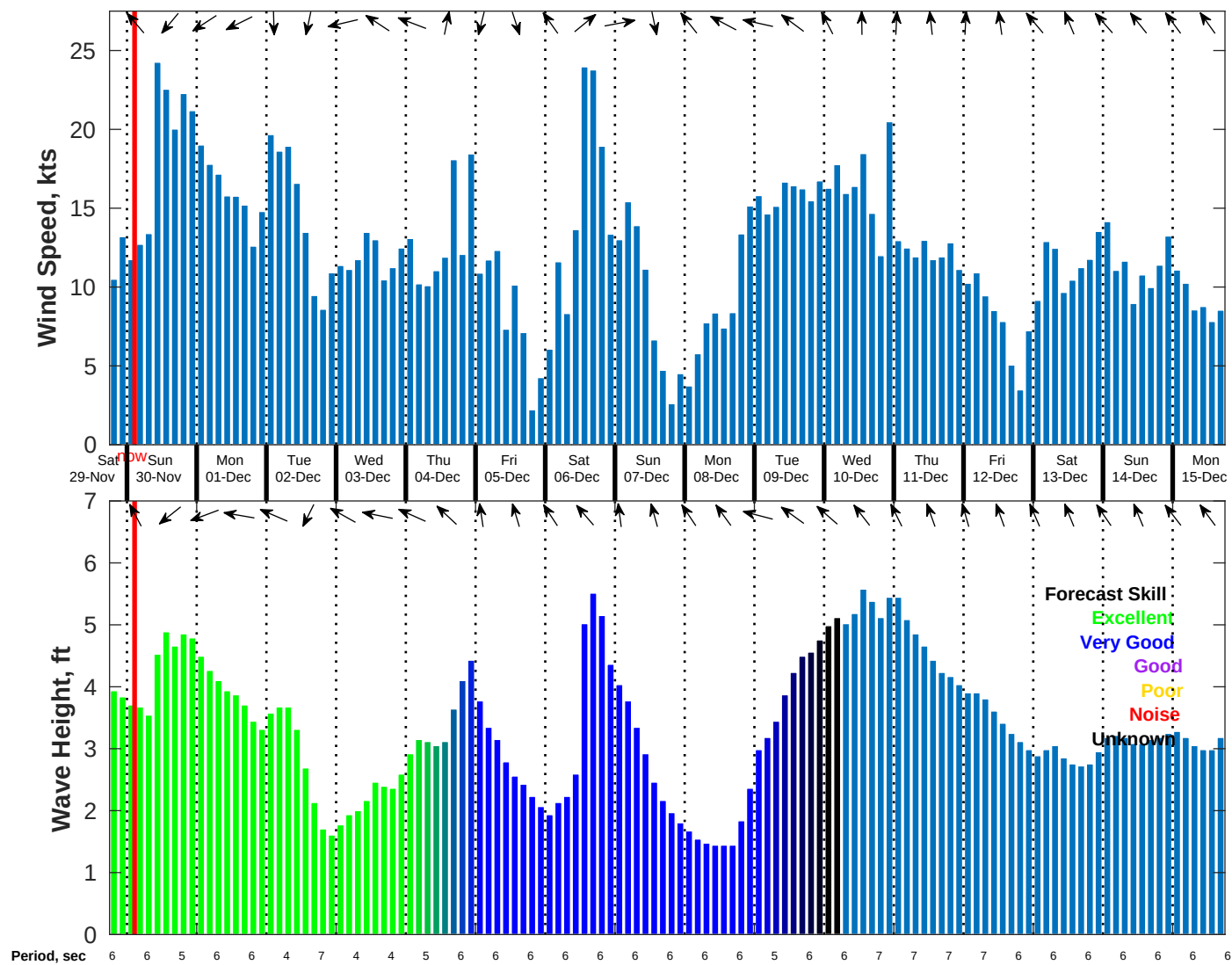
Wind & Wave Forecast for NDBC 42035 from 29-Nov-2025 18:00:00 to 15-Dec-2025 18:00:00
